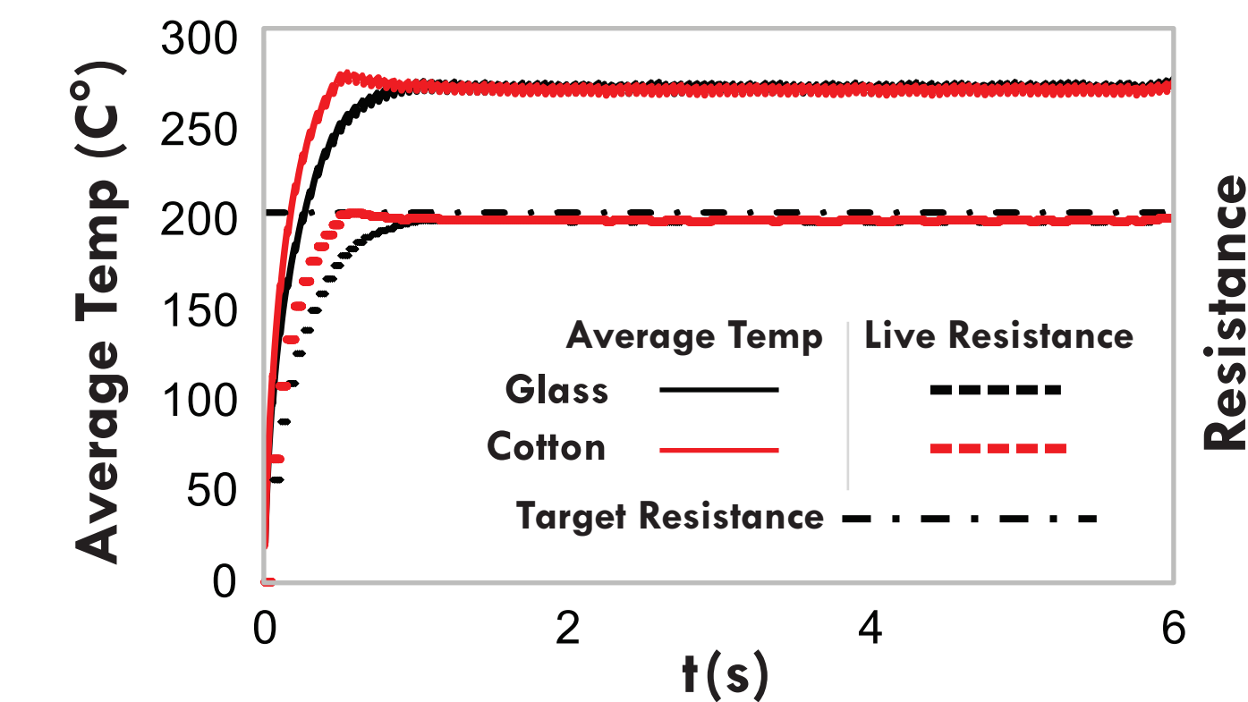
Figure 6. Temperature Regulation
