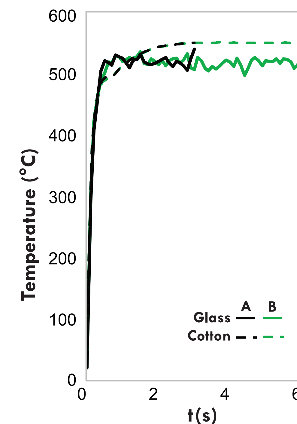
Figure 5. Unregulated Temperature
