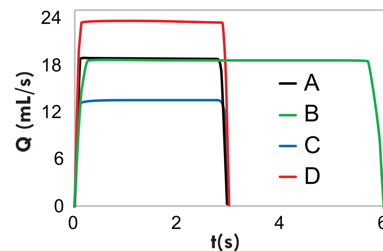
Figure 2. Puff Profiles
